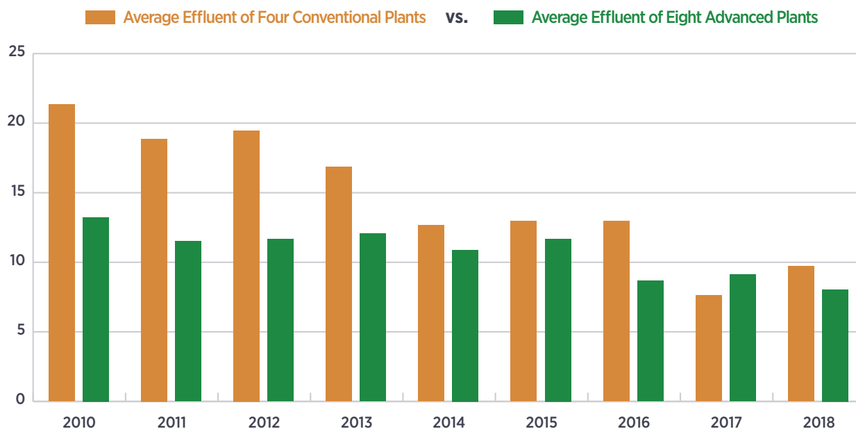
Average TN Concentration (mg/L)
